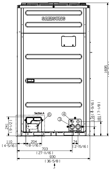
View C
