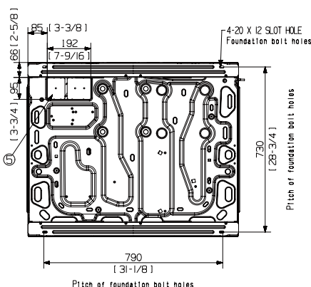
View C
