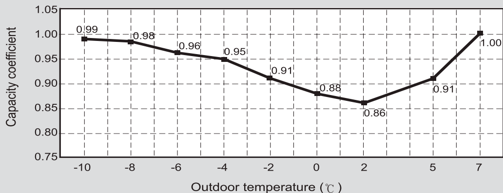
Capacity coefficient of outdoor unit on defrost operation
