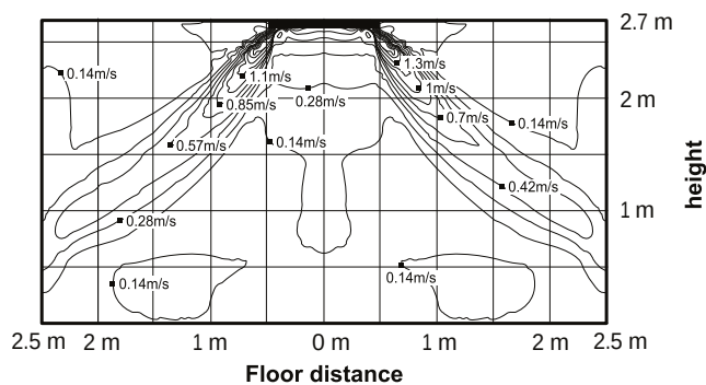
(3) Heating air velocity distribution
