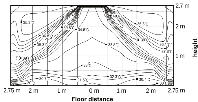
(4) Heating temperature distribution Discharge angle: 52°
