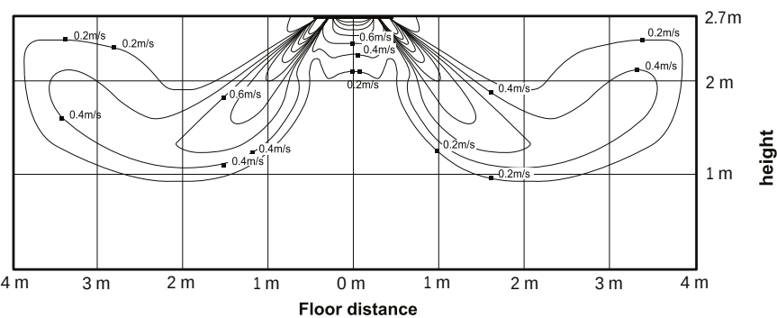
(3) Heating air velocity distribution Discharge angle: 52°
