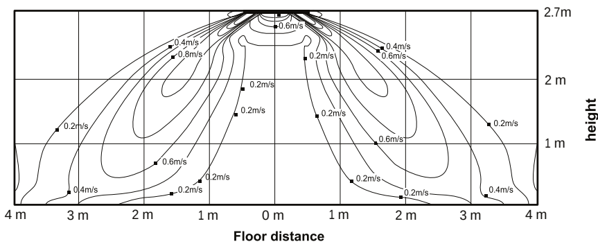
(1) Cooling air velocity distribution Discharge angle: 45°
