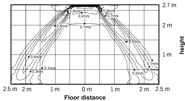
(1) Cooling air velocity distribution
