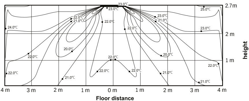
(2) Cooling temperature distribution Discharge angle: 45°
