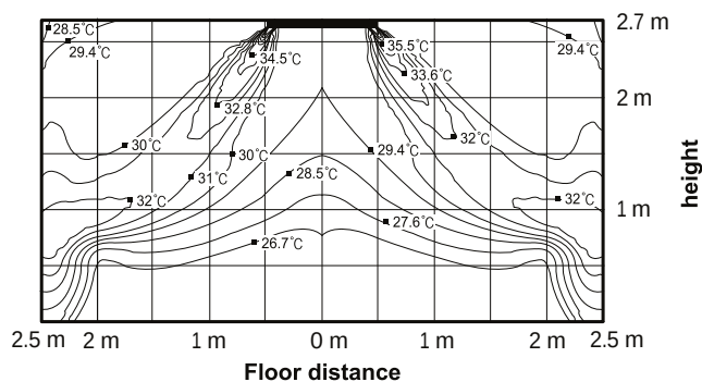
(4) Heating temperature distribution
