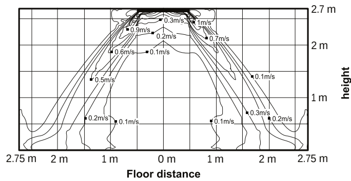
(1) Cooling air velocity distribution Discharge angle: 45°
