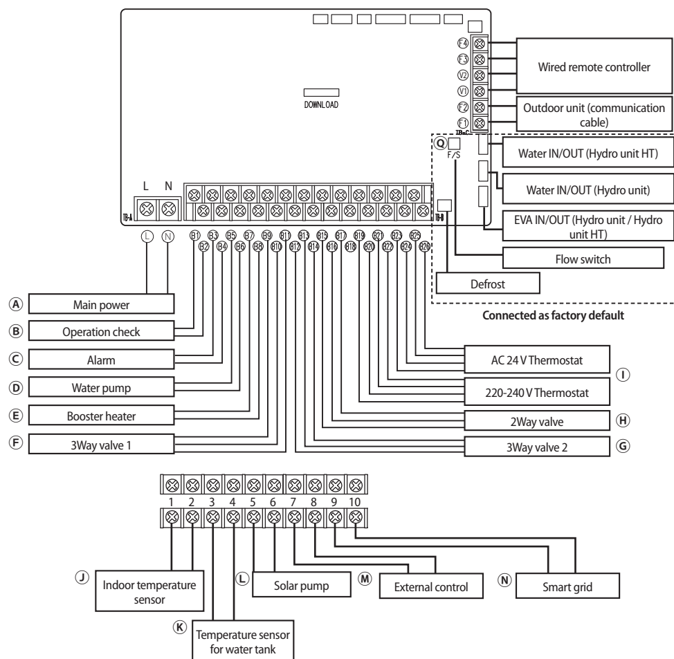
External contact connection diagram
