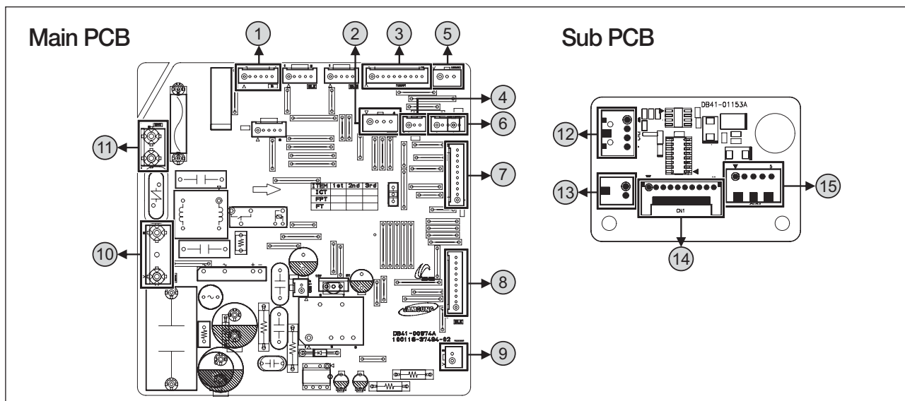
Main PCB
