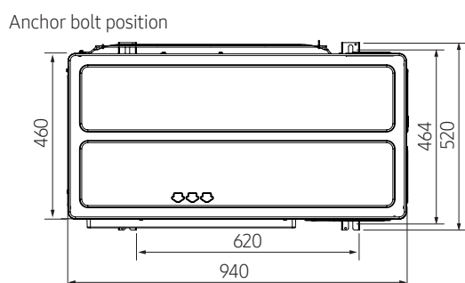
AM100/120BXMWGHX
