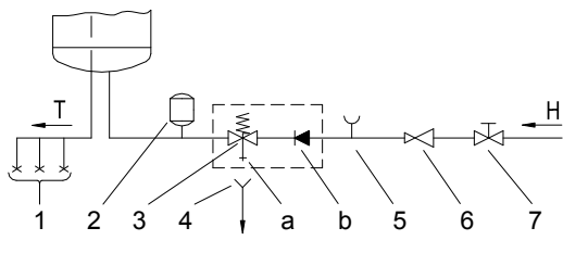
Fig. 7: Lukket system (under tryk)
