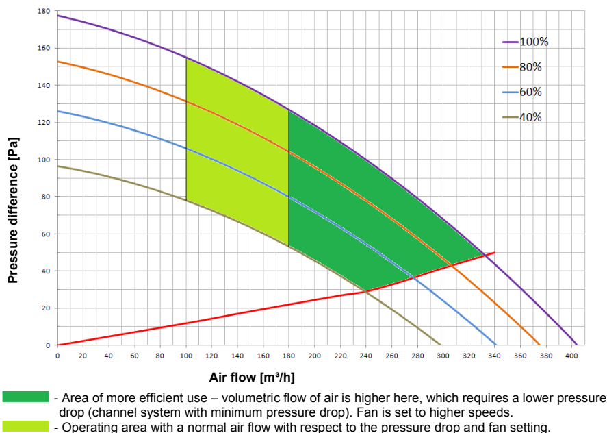
Diagram 1: Aerodynamic characteristics
