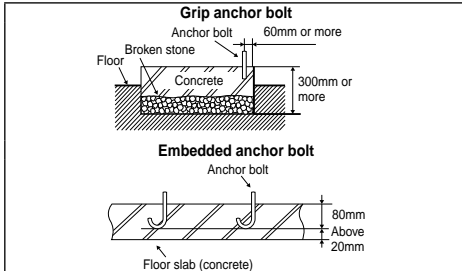
Illustration of grip type and embedded type anchor bolt
