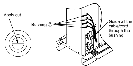
How to guide cable/cord to bushing
