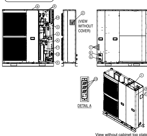
View without cabinet top plate
