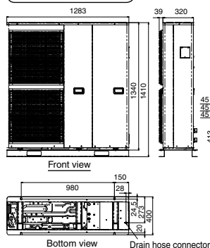
Dimension Diagram
