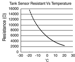
Graph 4.1: Tank sensor characteristic
