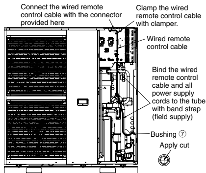
How to connect Remote Control to Provided Connector
