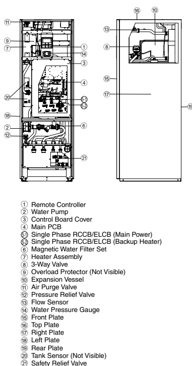
Main Components Diagram
