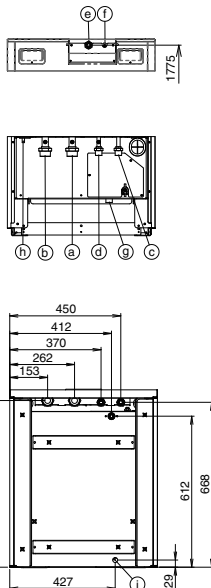
Tube Position Diagram
