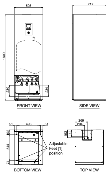
Dimension Diagram
