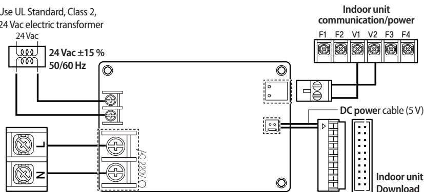
AC power for an indoor unit
