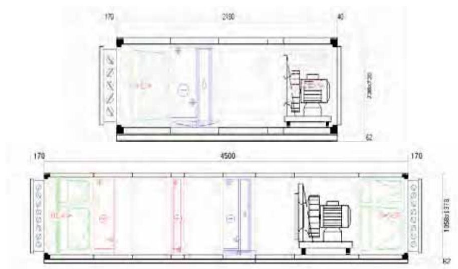
Hospital exhaust and supply units with run-around coil for energy recovery
