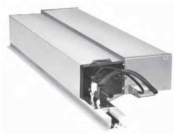
37AS: Air flow range: 19–78 l/s
